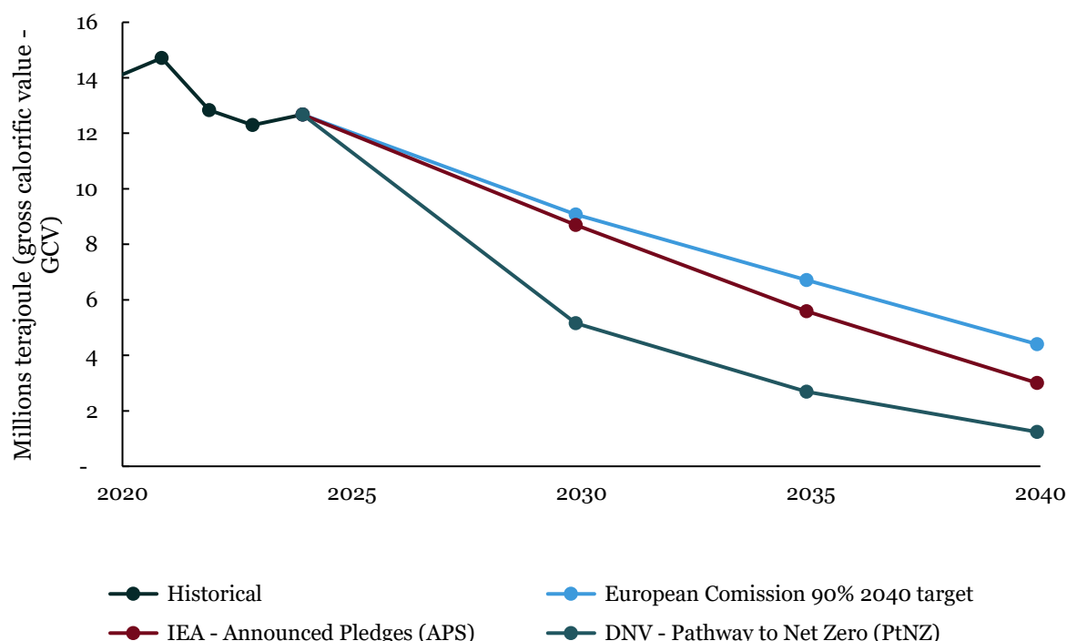
Figure 4-4: Natural gas demand in the EU in selected ambitious scenarios. Source: European Commission, IEA and DNV 49 50 51
